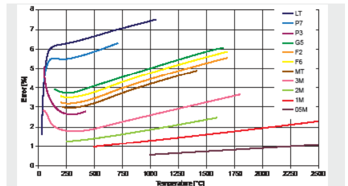
Measuring error in the case of emissivity wrongly adjusted by 10% as a function of the wavelength and object temperature (LT: 8 - 14 \mu\text{m} ; P7: 7.9 \mu\text{m} ; P3: 3.43 \mu\text{m} ; G5: 5 \mu\text{m} ; MT: 3.9 \mu\text{m} ; F2: 4.24 \mu\text{m} ; F6: 4.64 \mu\text{m} ; 3M: 2.3 \mu\text{m} ; 2M: 1.6 \mu\text{m} ; 1M: 1.0 \mu\text{m} ; 05M: 525 nm).
