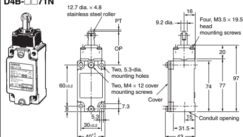
Top Roller Plunger D4B-□□71N
