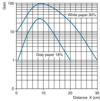
Diffuse reflective Models E3H2-DS30
