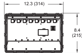
(MOUNTING CLIPS INSTALLED)
