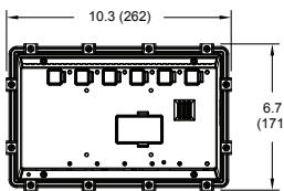
(MOUNTING CLIPS INSTALLED)
