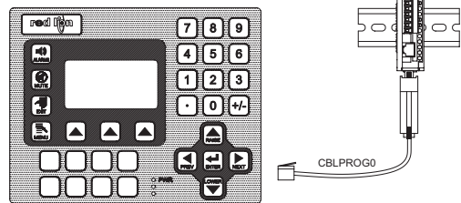
CONNECTING A G303 OPERATOR INTERFACE TO AN ICM5
