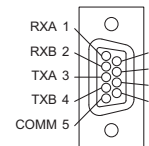
RS-485 (4-wire) DB9-F
