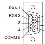
RS-485 (2-wire) DB9-F
