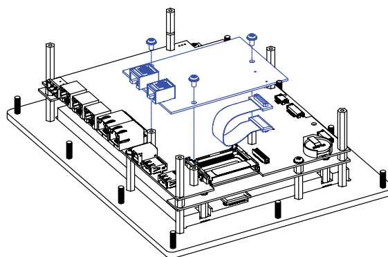
TYPICAL EXPANSION CARD INSTALLATION
