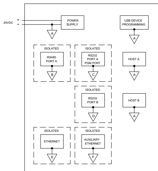
POWER SUPPLY ISOLATION BLOCK DIAGRAM (G308A2 ONLY)
