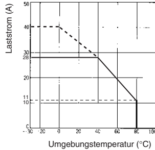
G3PA-450B-VD-2
