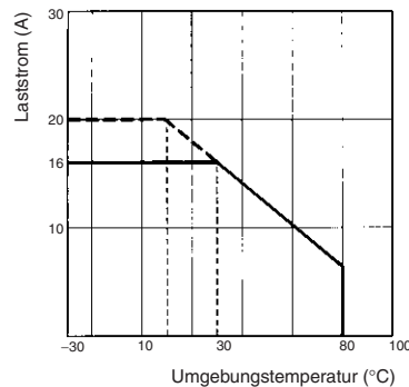
G3PA-450B-VD-2
