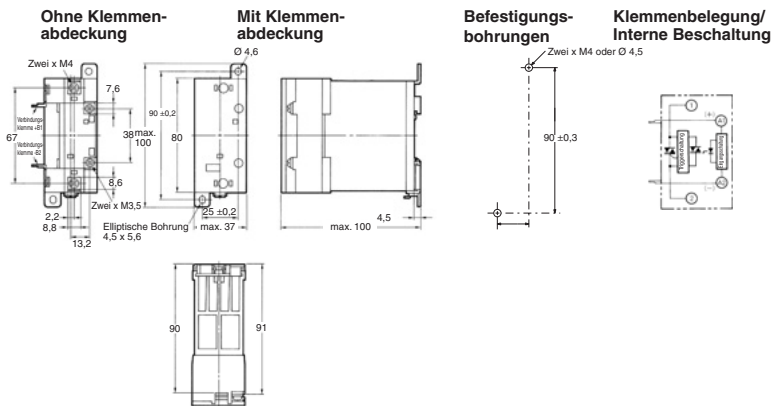
G3PA-430B-VD, G3PA-430B-VD-2
