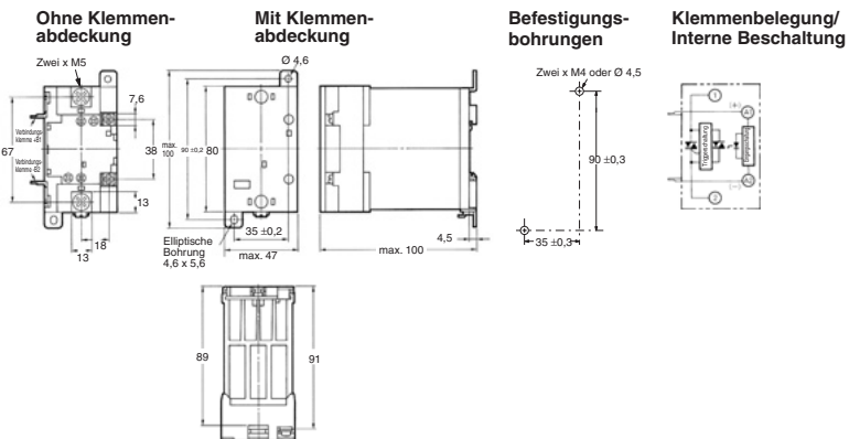
G3PA-430B-VD, G3PA-430B-VD-2
