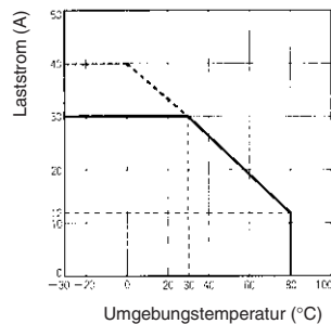
G3PA-430B-VD, G3PA-430B-VD-2
