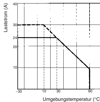
G3PA-430B-VD, G3PA-430B-VD-2
