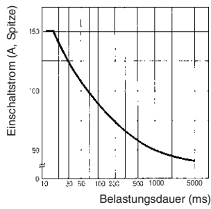
G3PA-210B(L)-VD
