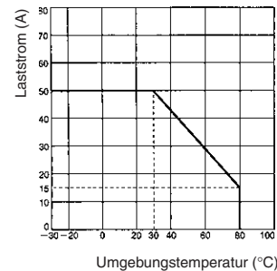
G3PA-450B-VD-2
