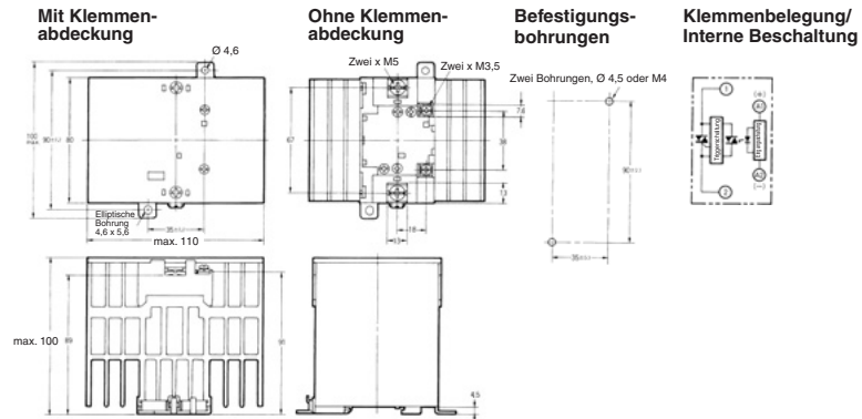
G3PA-260B(L)-VD G3PA-450B-VD-2
