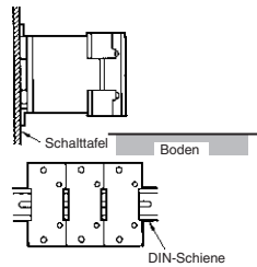
G3PA-210B(L)-VD, G3PA-220B(L)-VD
