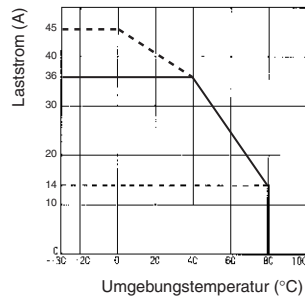
G3PA-430B-VD, G3PA-430B-VD-2
