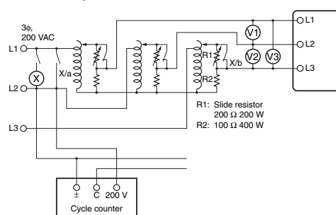
Connection Diagram
