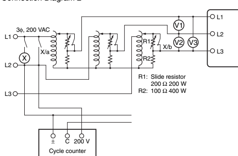
Connection Diagram 2
