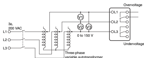
Connection Diagram
