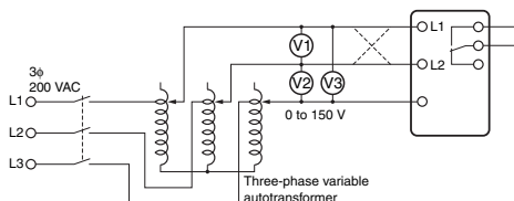
Connection Diagram 1
