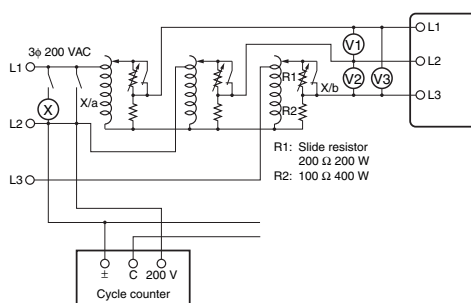
Connection Diagram 2
