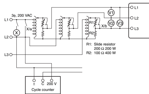
Connection Diagram 2
