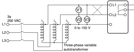
Connection Diagram 1
