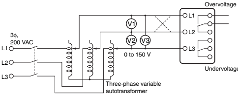
Connection Diagram 1
