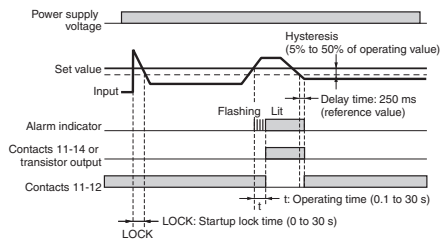
Overcurrent Operation Diagram (Output Drive Method: Normally Open) DIP switch setting: SW3 OFF, SW4 OFF
