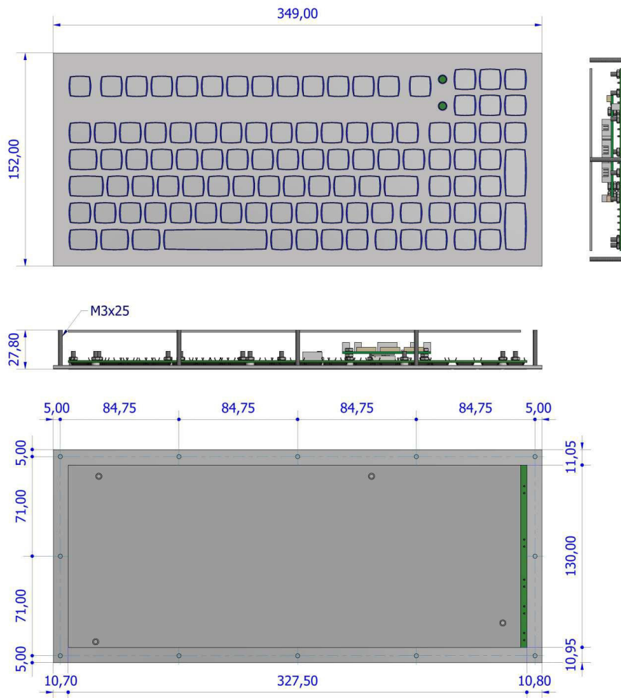
DIMENSIONAL DRAWING Panel mount version
