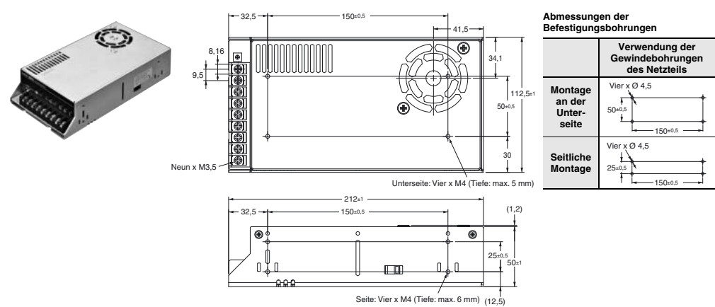
S8FS-C350□□ (350 W)
