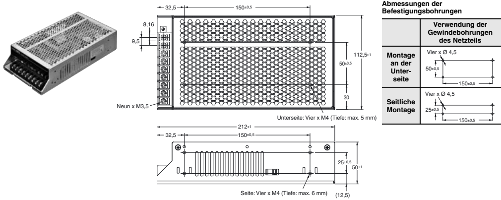
S8FS-C200□□ (200 W)
